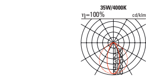
ONEline 1.2 INTENS NOT Systemleuchte
