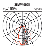
ONEline 1.2 INTENS NOT Systemleuchte
