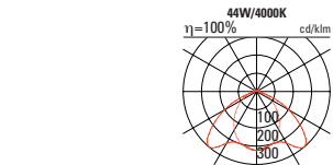
ONeline 1.5 BATWING NOT Systemleuchte
