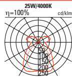
ONEline 1.2 OfficeMini Systemleuchte
