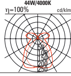
ONEline 1.5 OfficeMini NOT Systemleuchte
